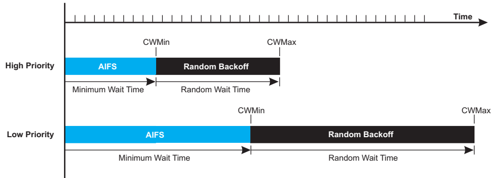
Figure 48 WMM Backoff Times
