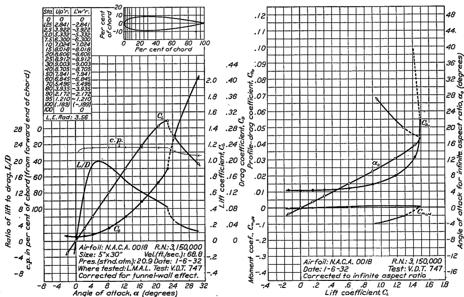
FIGURE 8.—N.A.C.A. 0018 airfoil.
