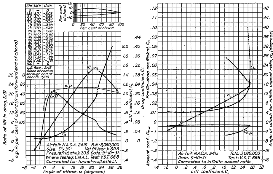
FIGURE 19.—N.A.C.A. 2415 airfoil.
