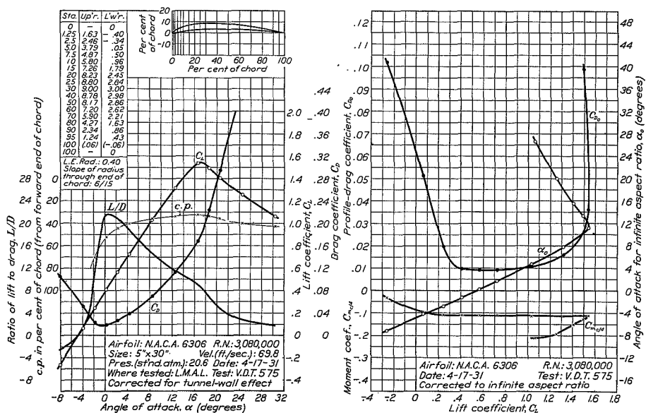
FIGURE 52.—N.A.C.A. 6306 airfoil.
