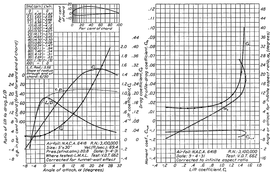
FIGURE 62.—N.A.C.A. 6418 airfoil.
