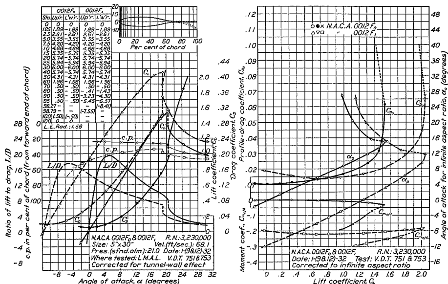
FIGURE 80.—N.A.C.A. 0012F0 and 0012F1 airfoils.
