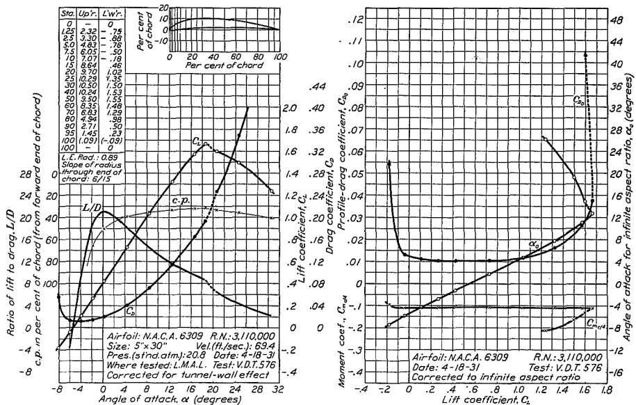
FIGURE 53.—N.A.C.A. 6309 airfoil.
