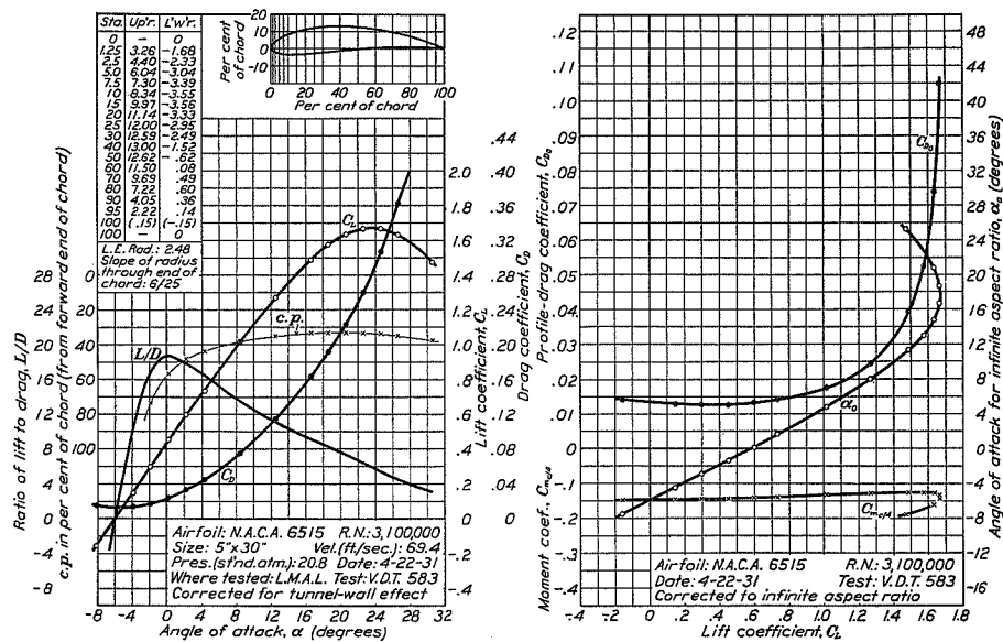
FIGURE 67.—N.A.C.A. 6515 airfoil.
