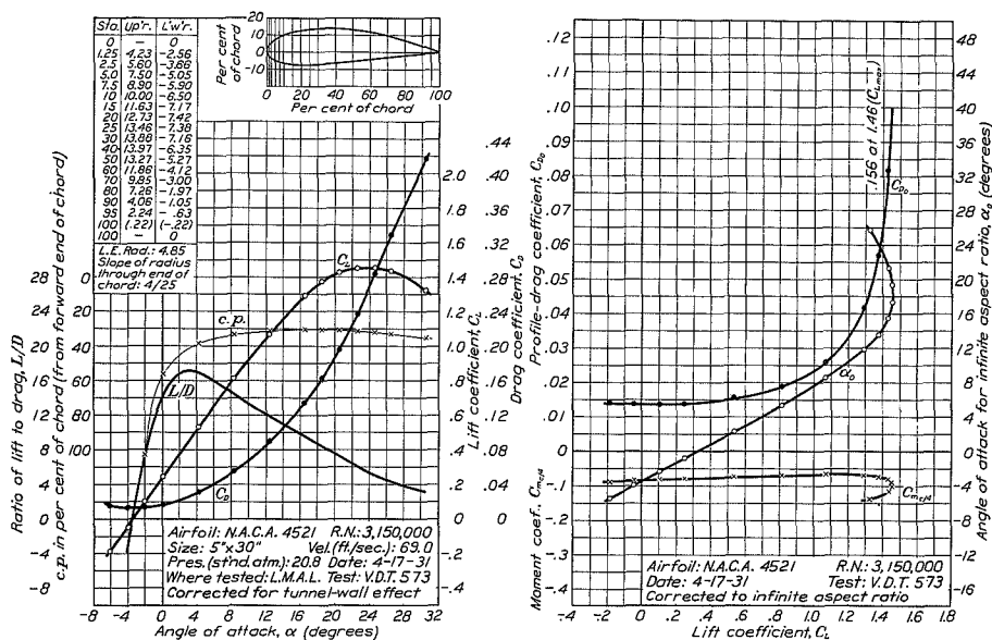
FIGURE 48.—N.A.C.A. 4521 airfoil.
