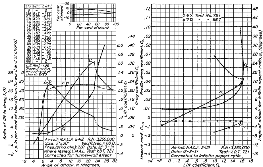
FIGURE 18.—N.A.C.A. 2412 airfoil.
