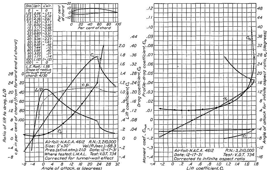
FIGURE 49.—N.A.C.A. 4612 airfoil.
