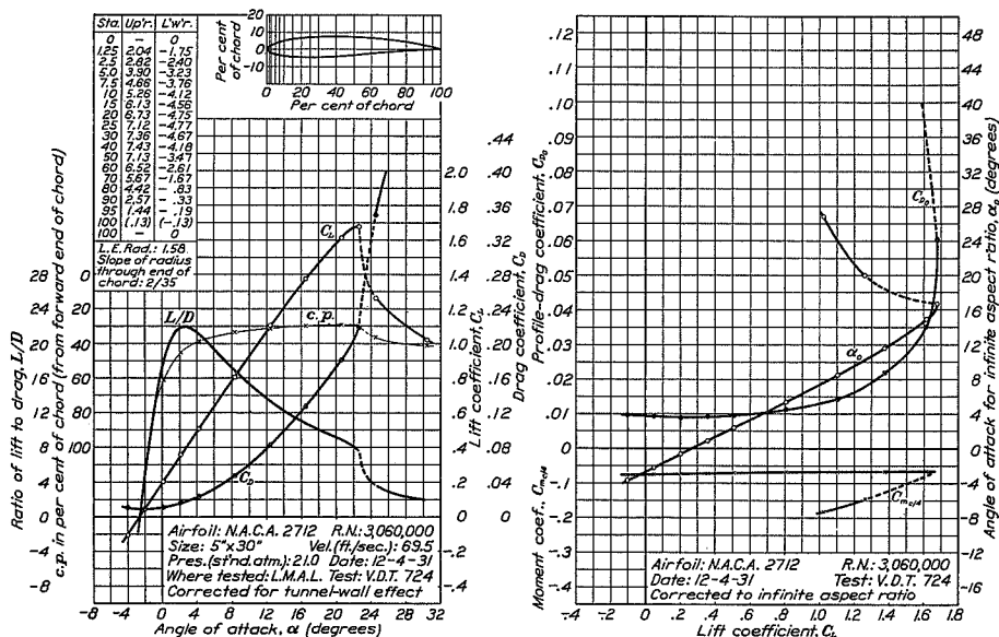
FIGURE 29.—N.A.C.A. 2712 airfoil.
