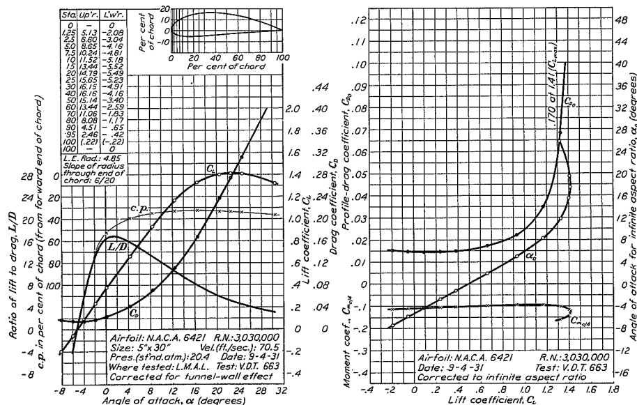
FIGURE 63.—N.A.C.A. 6421 airfoil.
