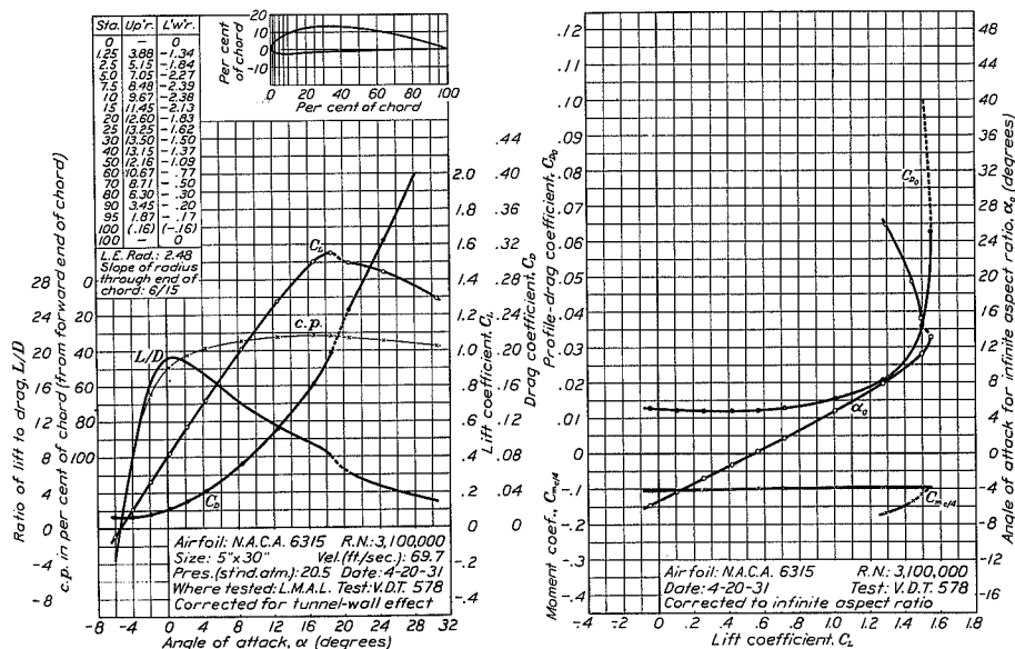
FIGURE 55.—N.A.C.A. 6315 airfoil.
