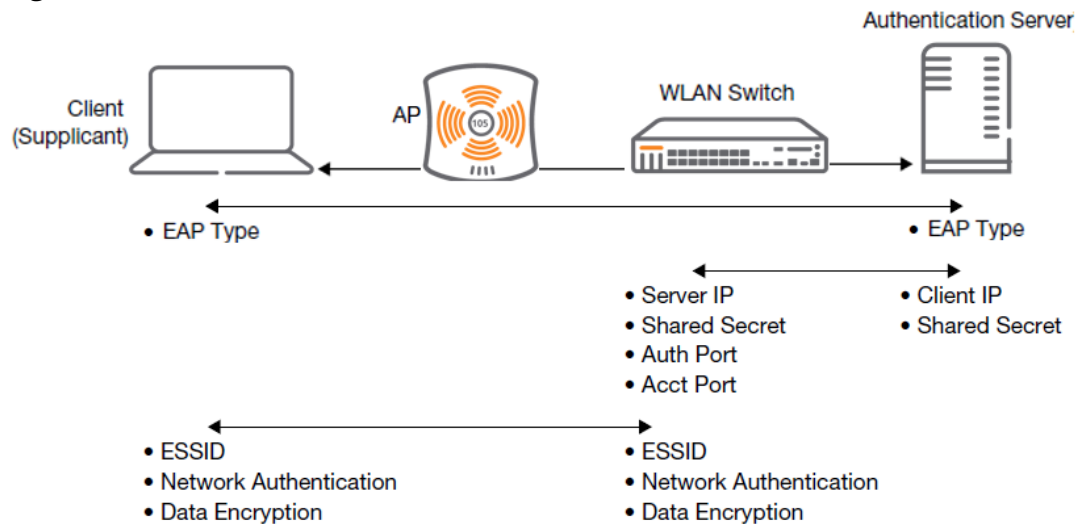
Figure 30 802.1X Authentication with a RADIUS Server
