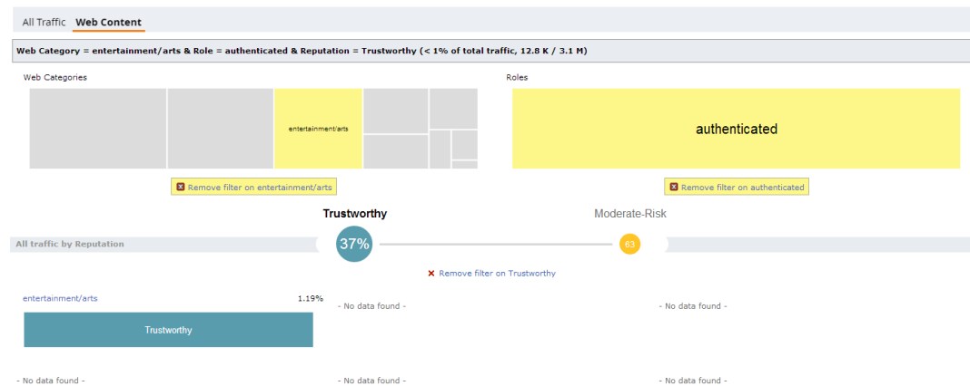
Figure 75 Multiple Filters
