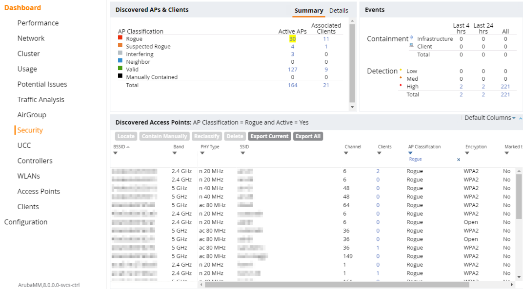
Figure 80 Security Page
