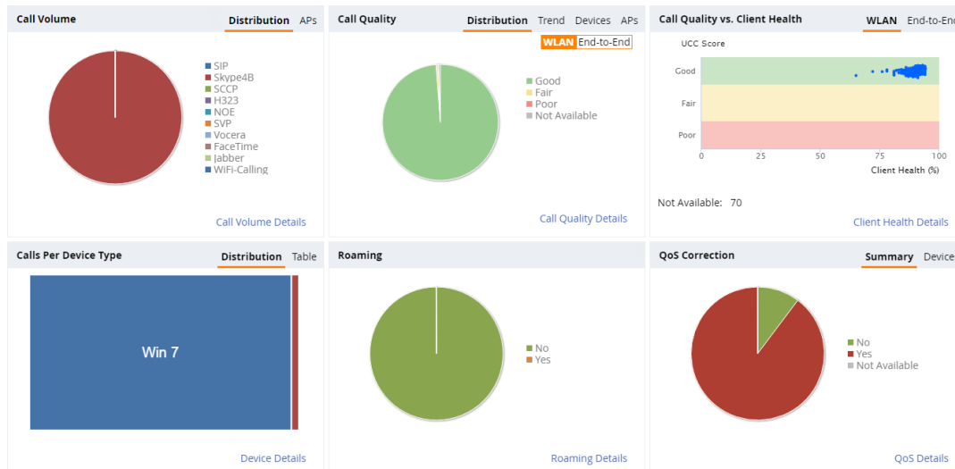
Figure 81 UCC Dashboard
