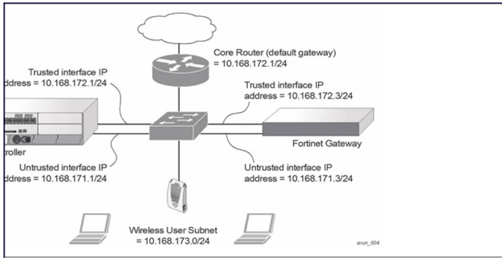
Figure 122 Example Route-Mode Topology
