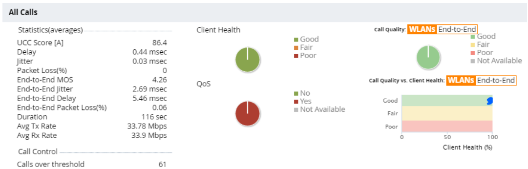
Figure 114 All Calls
