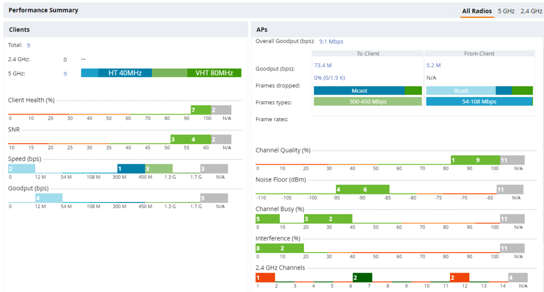
Figure 54 Performance Page
