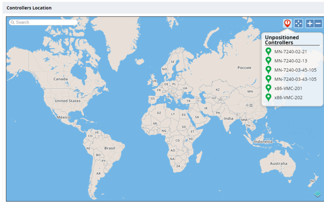
Figure 55 Network Page
