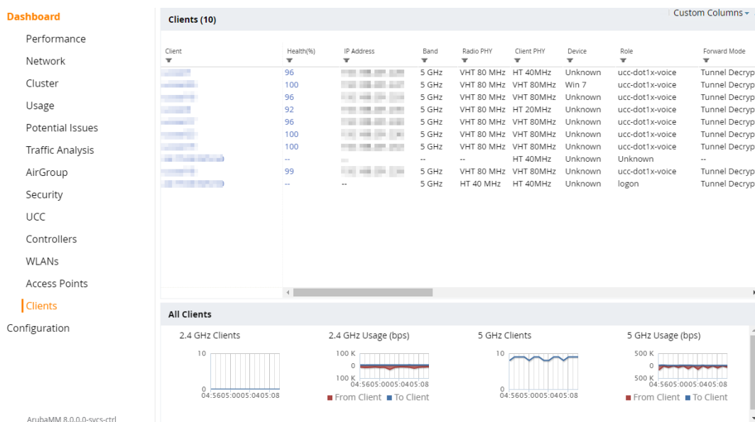
Figure 88 Clients Page
