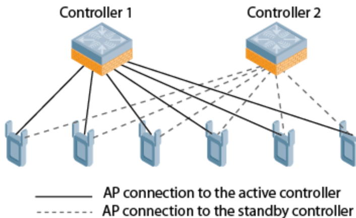
Figure 41 1:1 Active/Standby Deployment
