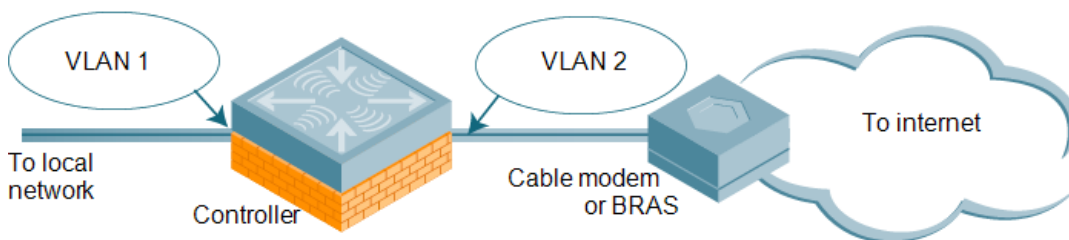
Figure 14 IP Address Assignment to VLAN via DHCP or PPPoE
