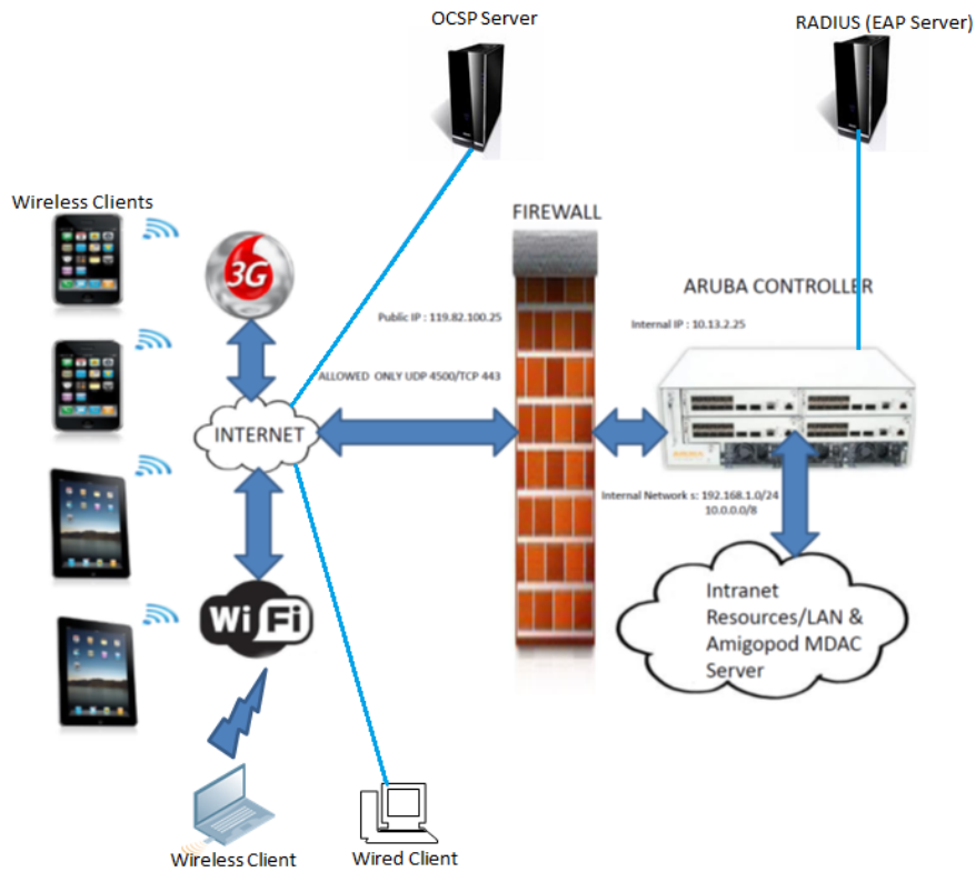
Figure 52 VIA Topology
