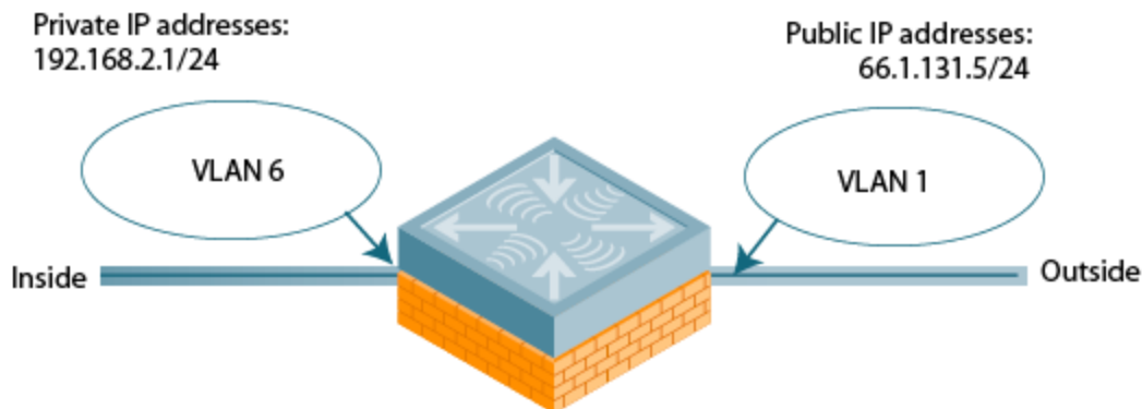
Figure 13 Example: Source NAT using the Managed Device's IP Address
