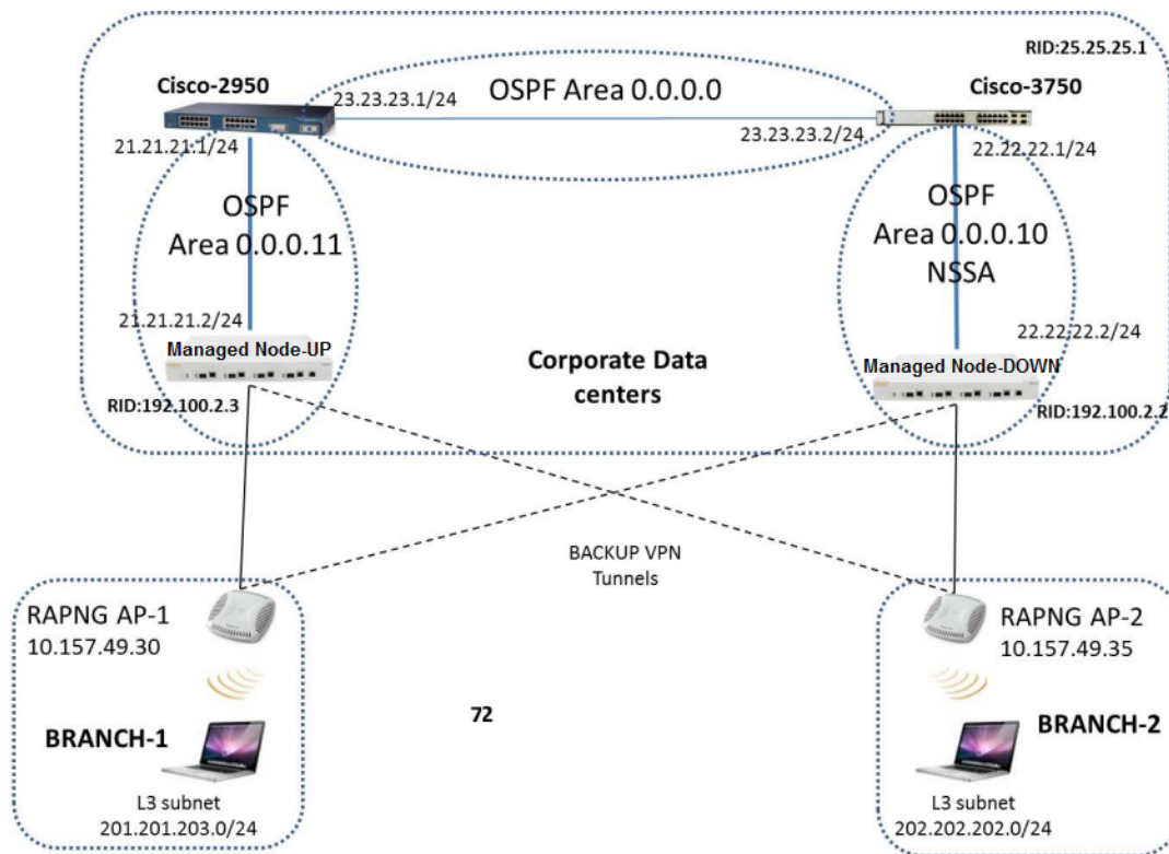
Figure 21 Managed Device Not-So-Stubby-Area (NSSA) and Normal Area
