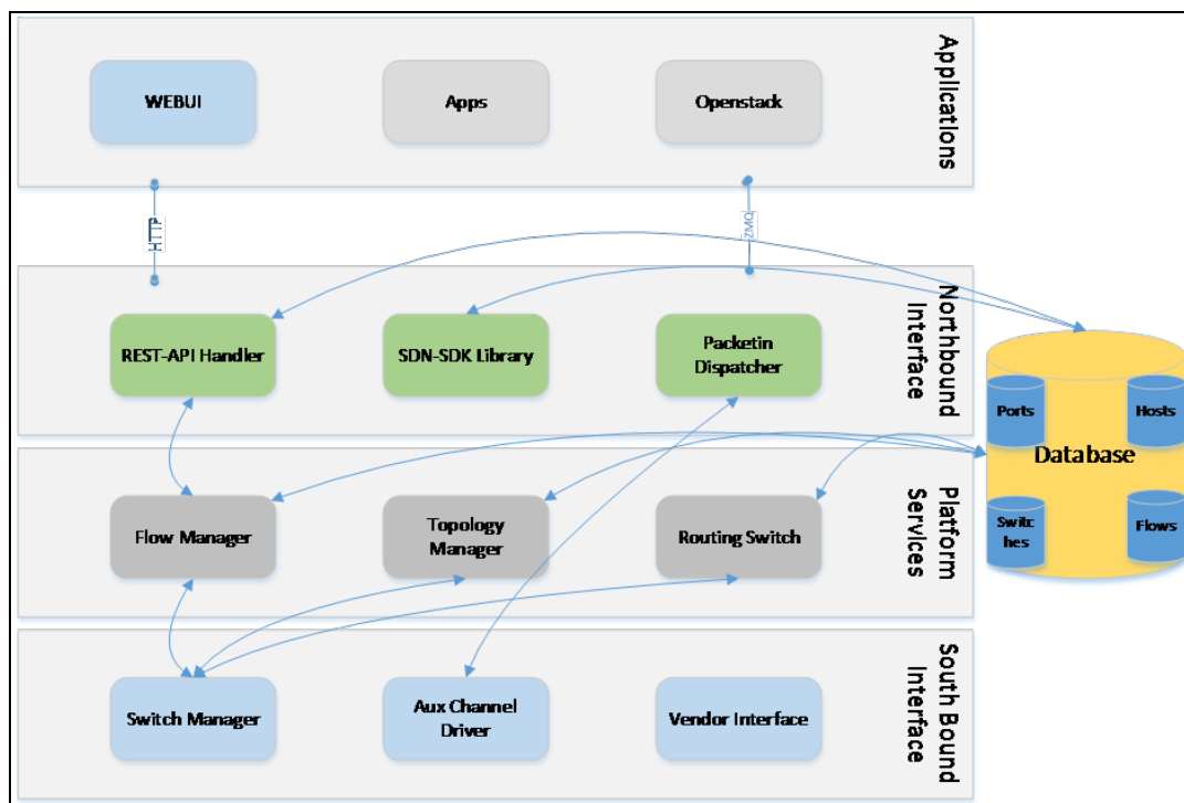
Figure 105 SDN Controller Architecture
