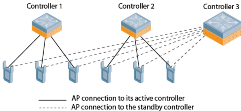
Figure 42 1:1 Active/Standby Deployment
