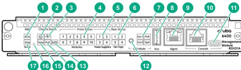
Figure 9 Management module features
