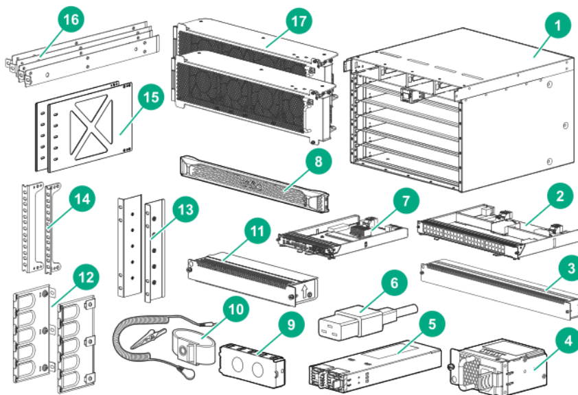
Figure 16 Hardware components
