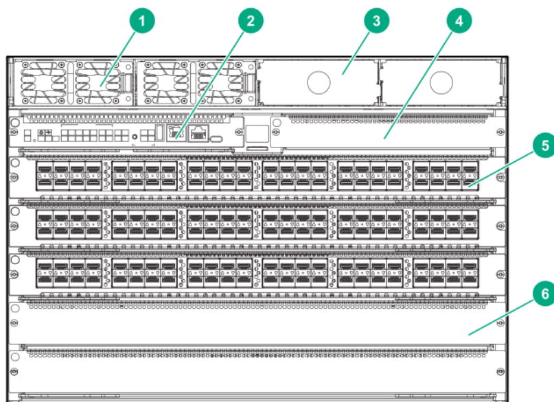
Figure 7 HPE Aruba Networking 6405: front of the switch
