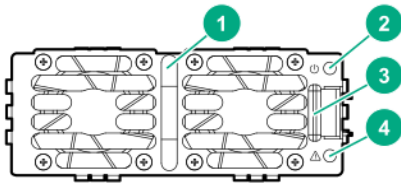
Figure 10 HPE Aruba Networking 6400 3000W Power Supply (R0X36A)
