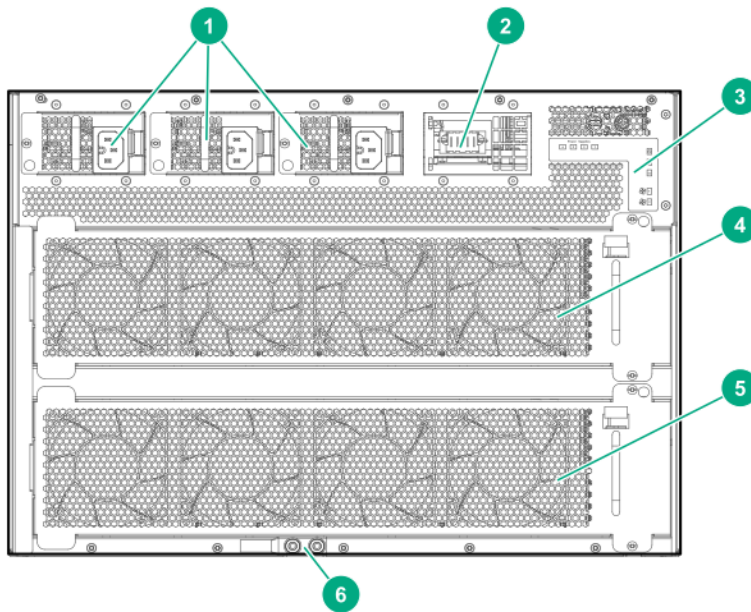
Figure 13 HPE Aruba Networking 6405 rear panel
