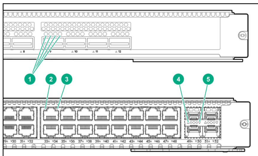
Figure 12 Line module LEDs
