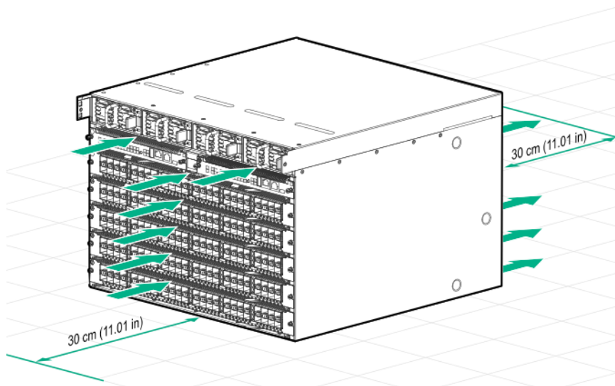
Figure 6 HPE Aruba Networking 6410 Switch Cooling Air Flow
