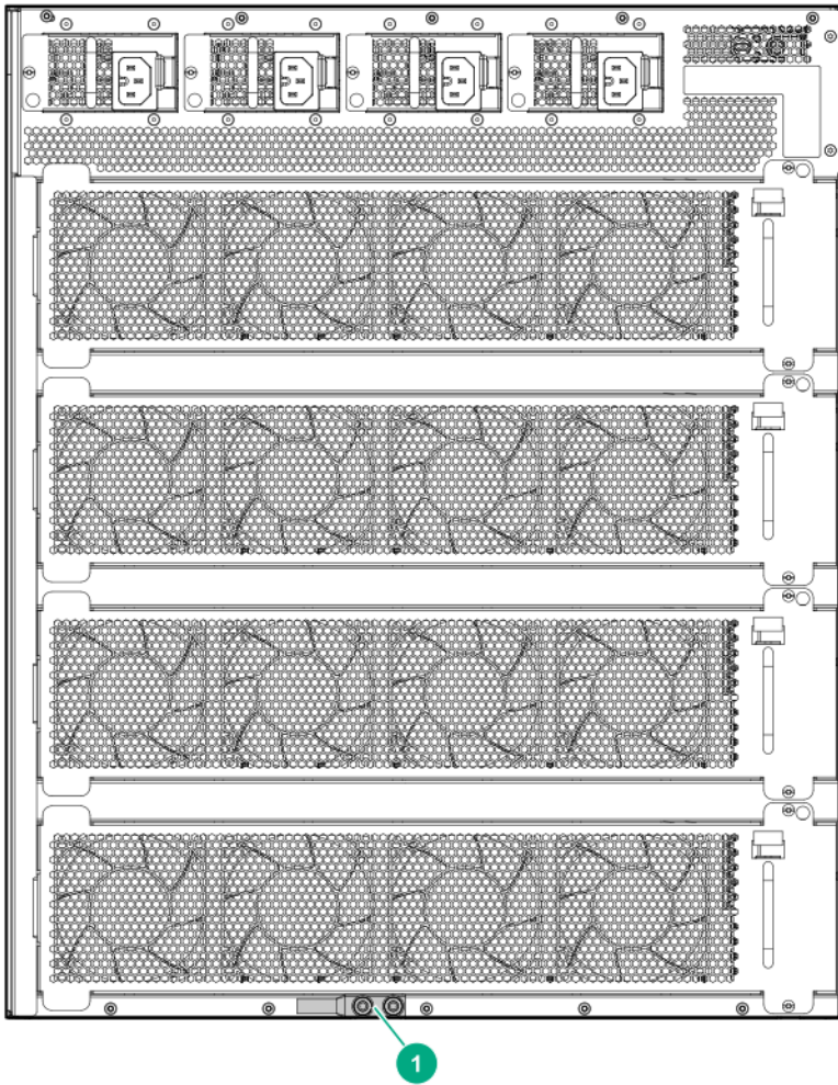
Figure 4 HPE Aruba Networking 6410 Switch grounding lug
