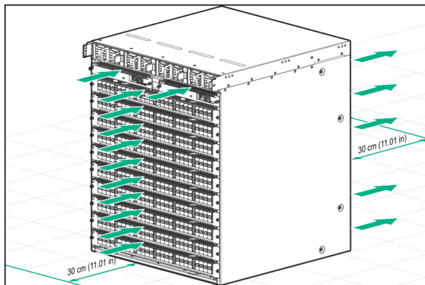
Figure 6 HPE Aruba Networking 6410 Switch Cooling Air Flow
