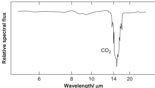
Figure 9.1 Part of the IR spectrum of Mars, with a prominent absorption line due to CO 2 . Note that the smooth shape of the spectral flux from an ideal thermal source at 273 K has been subtracted. (Adapted from C.A.Beichman, JPL Publication, 96-22, (1966))
