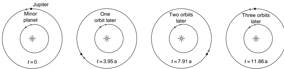
Figure 3.2 The 3:1 mmr of an asteroid with Jupiter. Figure 1.14 illustrates the 2:1 resonance.
