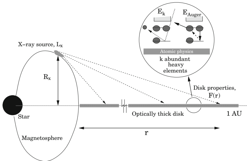
Fig. 8.5 Geometric set-up to calculate the X-ray ionization rate in protostellar disks. The assumption is that X-ray sources originate somewhere near the stellar magnetosphere \sim 10 R_\odot above the disk plane. The X-rays are characterized by the shape of the spectrum g(e) and the integrated X-ray luminosity L_x . Radiation hits somewhere in the middle of the optically thick disk at a distance of about 1 AU. The response then depends on the irradiated flux, atomic physics, and geometry. Adapted from Glassgold et al. [579]
