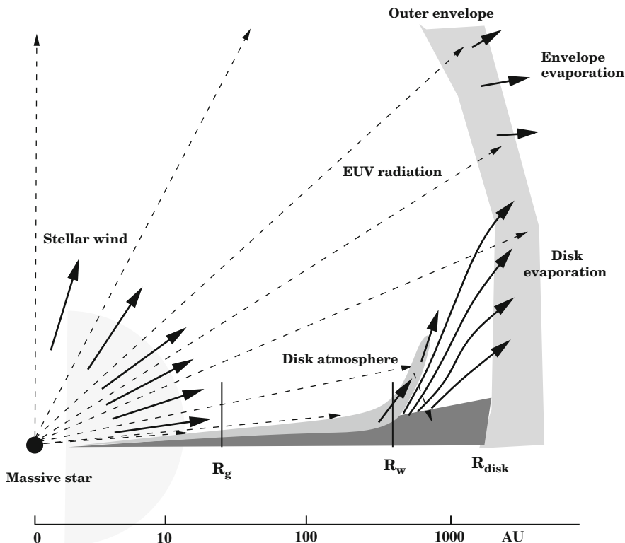
Fig. 8.8 Illustration of a system where the central massive star evaporates its immediate environment consisting a massive disk and maybe a residual outer envelope. In disk evaporation the ram pressure of the stellar wind pushes ionized atmospheric matter beyond the limit R_g where it is gravitationally bound until it is counterbalanced by thermal pressure. At this point matter is removed from the disk. Beyond R_w diffuse irradiation also causes disk evaporation. Similarly the EUV field and the ram pressure of the stellar wind will eventually disrupt any residual outer envelope
