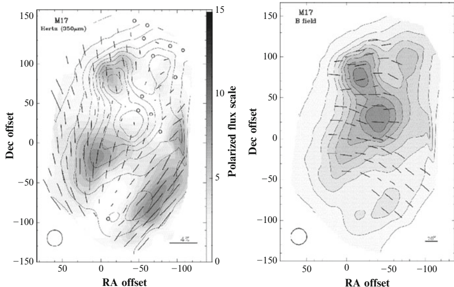
Fig. 4.7 ( left ) Polarization map of M17 at 350 \mu\text{m} . The center position is at R.A. = 18h17m314, Dec. = -16^{\circ}14'250'' (B1950.0). The contours show the continuum flux levels. The gray scale gives the polarized flux according to the scale on the right. The thick lines illustrate the direction of the polarization vectors. The large circle is the beam width. ( right ) Orientation of the reconstructed magnetic field in M17. The vectors show the projected orientation. The length of the vectors represent the viewing angle as scaled in the right corner giving some 3-D information. From Houde et al. [234]
