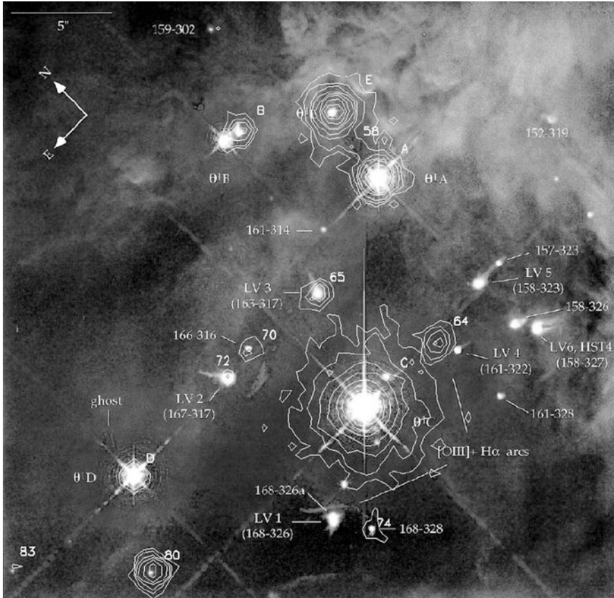
Fig. 12.3 X-ray contours from observations of the Orion Trapezium obtained by Chandra overlaid onto an optical HST observation. The field of view is 30 \times 30 arcsec 2 and the contours represent total X-ray flux levels. Credit: HST image by J. Bally [1159]/NASA; Chandra contours by Schulz et al. [532]
