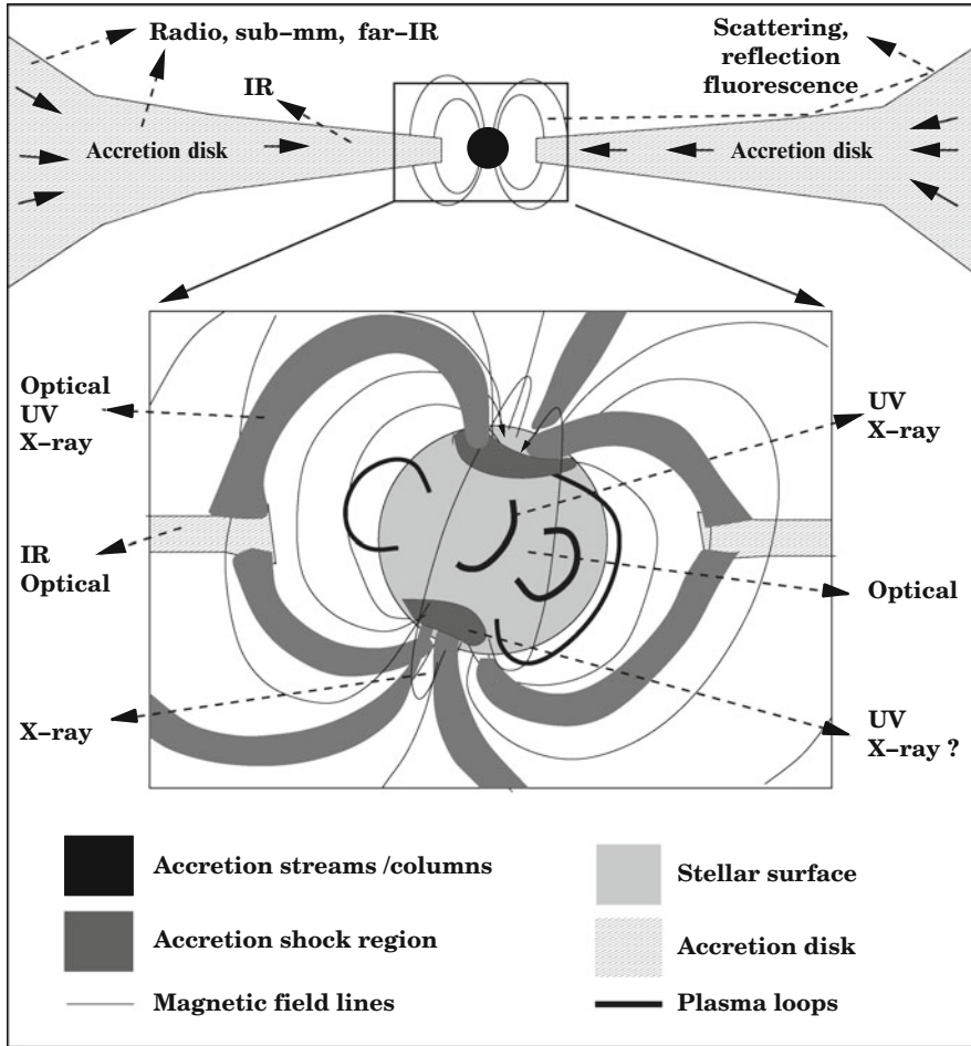
Fig. 6.14 Schematic impression of a classical T Tauri stellar environment. Dominant in size ( \sim 100 AU) is an accretion disk. The circumstellar disk emits at radio, mm, sub-mm, and far-IR wavelengths. The accretion disk itself radiates at IR, specifically near 1\text{--}5\ \mu\text{m} . The radiation from the central source at shorter wavelengths may reflect and scatter at the circumstellar disk. The local environment of the PMS star is characterized by the interaction of the turbulent magnetic field with the inner accretion disk. The stellar magnetic field not only disrupts the inner disk (at \sim 0.1 AU), but creates accretion streams and columns onto the stellar surface, which may produce accretion shocks. Accretion streams will emit broad-line emission from optical (i.e., H Balmer lines) to X-rays (i.e., O, Ne, Mg, Lyman \alpha ). Hot accretion shocked regions may produce continuum emission. The latter has no effect on the effective temperature of the surface, which thus radiates an optical blackbody spectrum. The near stellar magnetic field creates a hot stellar corona, similar to the one observed in the Sun, but with X-ray fluxes that are 1,000 times stronger. Explosive high-energy emission has its origin in magnetic reconnections, which could be caused by rotational twists of the turbulent magnetic field lines
