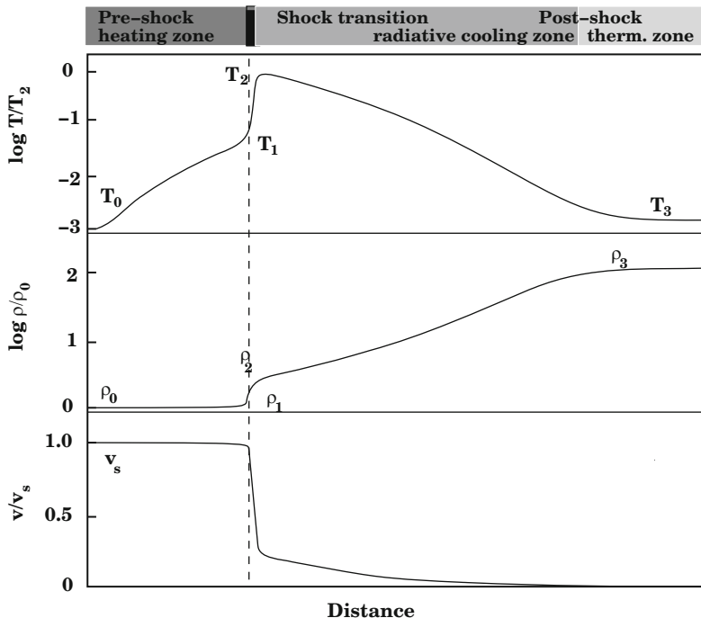
Fig. 3.8 Temperature, density, and velocity dependence of a strong shock in a single fluid flow distinguishing between three shock zones: the pre-shock with radiative heating, the shock transition zone with jumps in temperature, density and velocity, and the post-shock zone which is cooling radiatively. Adapted from Draine and McKee [93]
