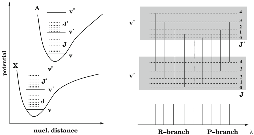
Fig. C.3 (left) Schematic illustration of locations and splittings of vibrational ( v ), rotational ( J ) and electronic ( A , X ) levels. The latter are shaped similar to Morse potentials. (right) Vibrational-rotational bands with transition of the R-branch (lines to the left of the J = 0 \leftrightarrow J' = 0 transition, which is actually forbidden) and the P-branch (lines to the right). Adapted from [1311]
