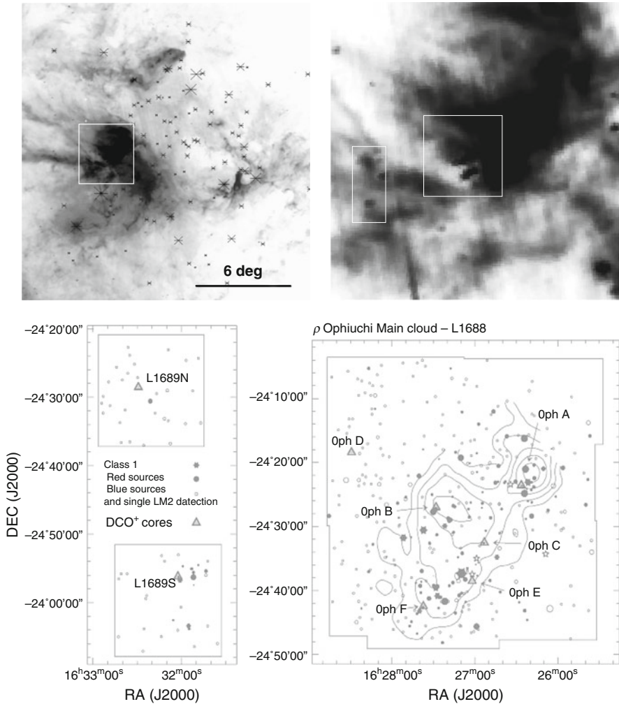
Fig. 11.10 The morphology and stellar content of the \rho Oph Cloud. The upper-left portion of the figure shows the IRAS large-scale view of the environment of the cloud, which is marked by the white square. The cloud is embedded into the Upper Scorpius region with a large association of OB stars (marked by asterisks). The upper-right portion shows the cloud zoomed in from the white square in the upper left image. There are no massive stars associated with the cloud itself. The cloud is fragmented into several subclouds and clumps. The diagram at the bottom shows the stellar and morphological content of the cloud (as marked in the upper-right image) as recently measured by S. Bontemps and colleagues using the ISOCAM on board ISO at mid-IR wavelengths. Filled stars mark Class I, filled circles Class II, and open circles are likely Class III YSOs. The contours show the extent of L1688 . Credits: upper-left image by T. Preibisch; bottom diagrams from Bontemps et al. [1097]
