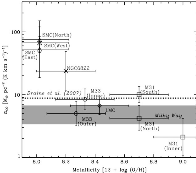
Fig. 3.10 The CO-to-H 2 mass ratio \alpha_{CO} as a function of metallicity for the Milky Way and galaxies of the local group (from Leroy et al. [96])
