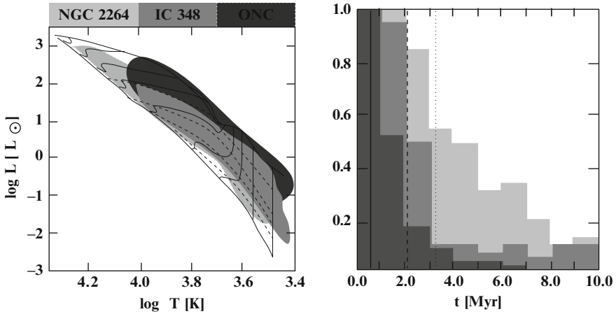
Fig. 11.5 ( left ) HR-diagrams of three very young embedded clusters. The shaded areas engulf the measured data. The data and HR tracks ( solid lines ) are taken from [1051]. The dashed lines are timelines. ( right ) The same data binned by time bins according to the tracks in the left HR-diagram and normalized to the maximum time bin. The solid vertical line marks the median age of the ONC . The dashed and dotted lines are for IC 348 and NGC 2264 , respectively. Adapted from Palla and Stahler [1051]
