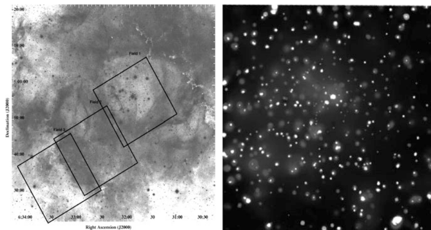
Fig. 4.21 (left:) Optical image of the center of the Rosette Nebula. The squares mark the fields covered by X-ray observations. (right:) X-ray image of field 1, the central region of the Rosette, obtained with the Chandra X-ray Observatory. Besides the many bright X-ray sources in the field of which many are O-stars there is strong diffuse emission present indicating the existence of hot plasma and thus high ionization. From Townsley et al. [310]
