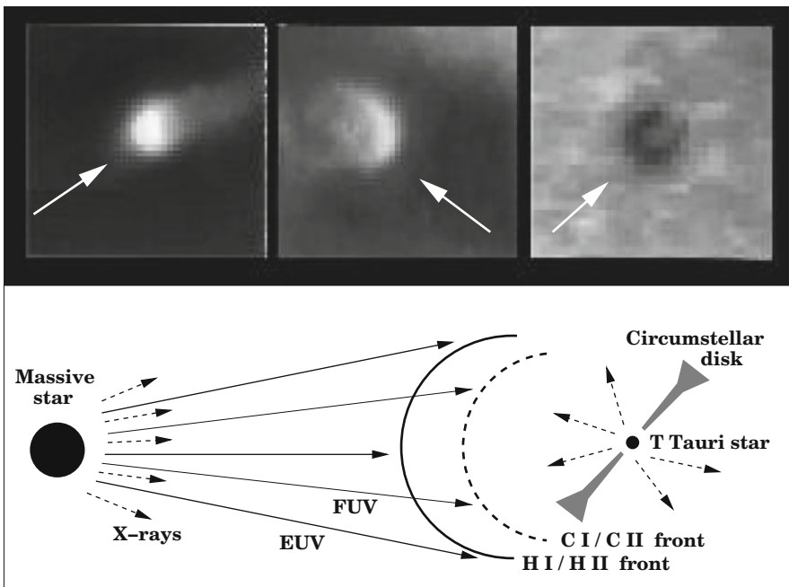
Fig. 12.2 ( top ) The panel shows three Orion proplyds observed with HST in 1992. The white arrows indicate the direction of the ionizing radiation from the massive Trapezium Stars specifically \Theta^1 Ori C [1151]. Credit: C.R.O'Dell and NASA. ( bottom ) The sketch illustrates how ionizing radiation from a massive star interacts with nearby protostellar disks primarily through EUV and FUV radiation. Though the massive star is a strong X-ray emitter ionizing effects on the proplyd is unknown. X-rays have been detected from the central T Tauri star (see Fig. 12.3)
