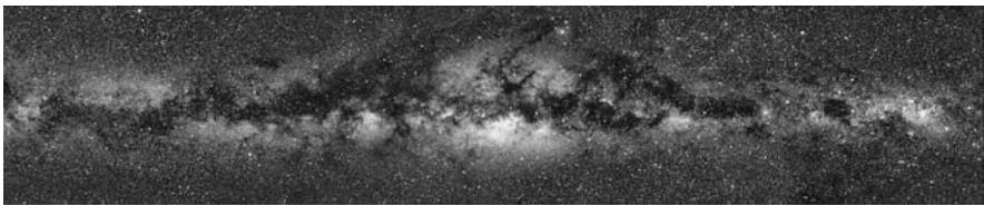
Fig. 3.20 Dust in the southern Milky Way. Credit: Photography by A. Mellinger; from http://home.arcor-online.de/axel.mellinger
