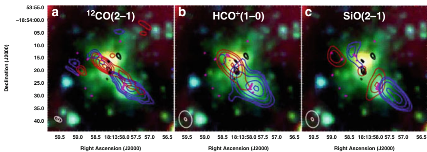
Fig. 9.9 Three-color Spitzer images (3.6, 4.5, 8.0 \mu\text{m} : blue, green, red) of the EGO G11.92-0.61 containing hot cores and outflows. The images are overlaid with contours of 1.4 mm continuum emission (black) and high velocity (a) ^{12}\text{CO} , (b) \text{HCO}^+ , and (c) SiO emissions. Positions of 6.7 GHz \text{CH}_3\text{OH} masers are marked with black diamonds; positions of 44 GHz \text{CH}_3\text{OH} masers are marked with magenta crosses (from Cyganowski et al. [772])
