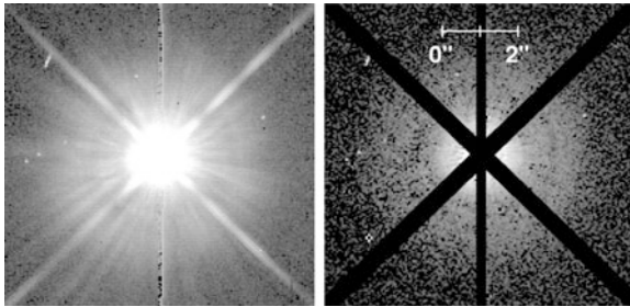
Fig. 8.1 Hubble WFPC2 images of the close CTTS TW Hya. The left image shows the raw image, the right image the same but with instrumental distortions subtracted. The residual image shows the face-on disk of the stars. From Krist et al. [552]
