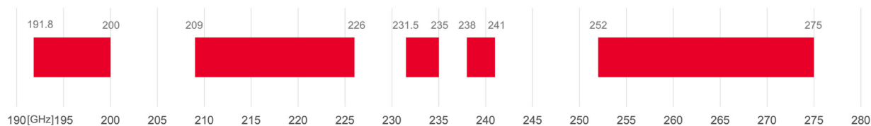
Figure 4. Simplified global allocation for mobile / fixed frequency allocation, 92 to 175 GHz
